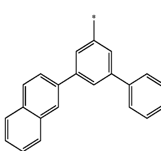
Formula 3-10
