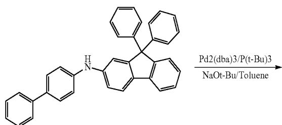
Intermediate 1-3
