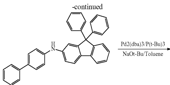
Intermediate 1-3
