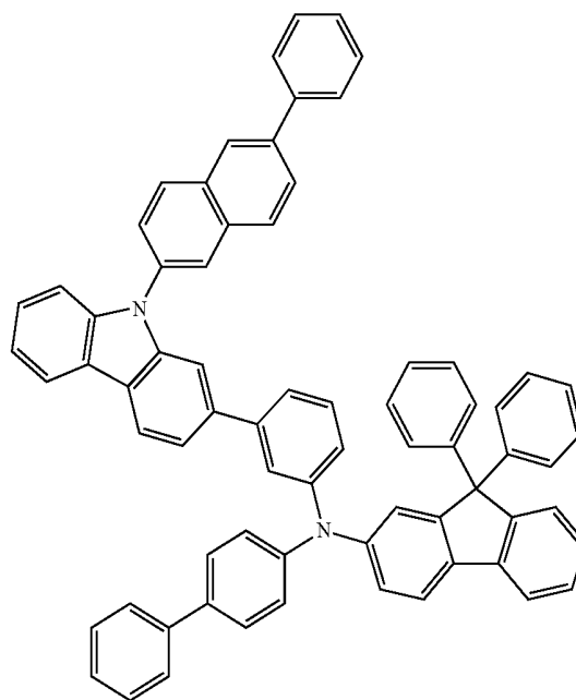
Compound 4
