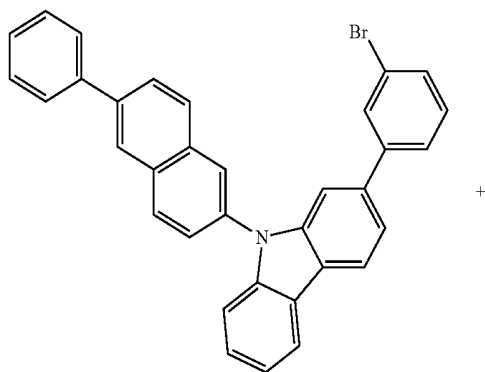
Intermediate 4(3)
