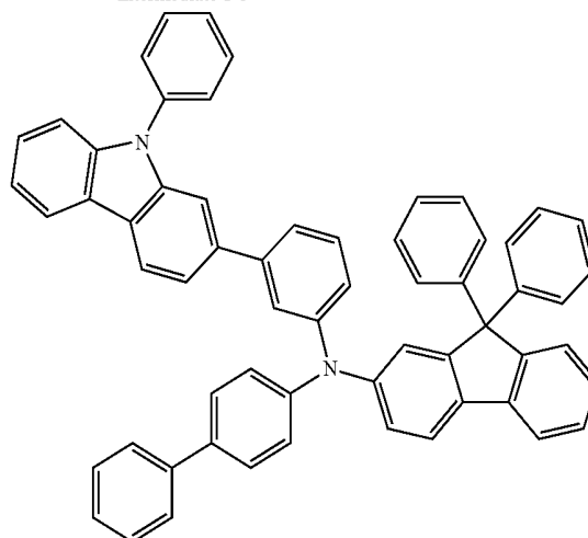
Compound 6
