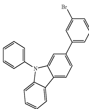
Intermediate 6(3)
