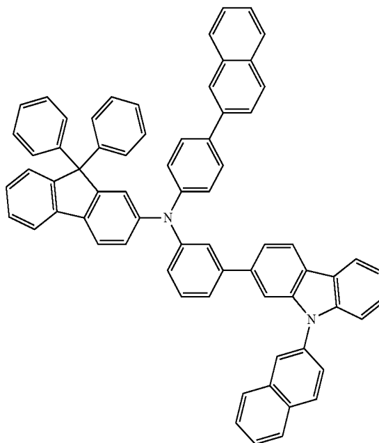
Formula 3-18
