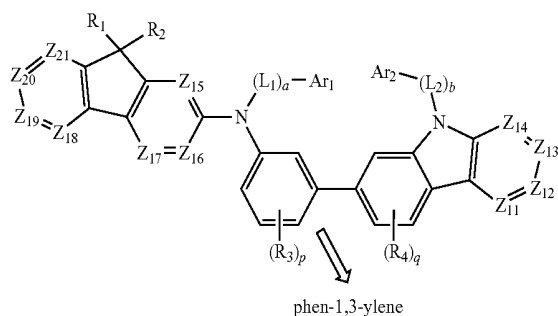
Formula 1'
