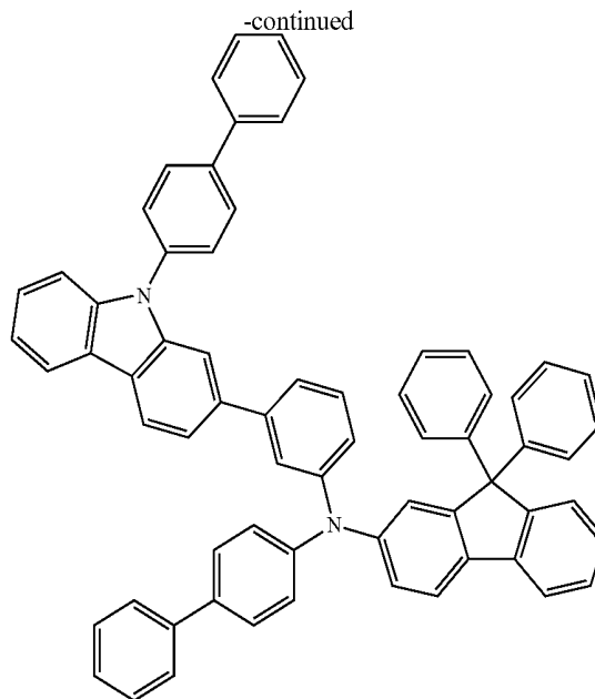
Compound 7
