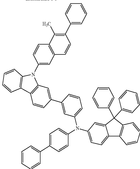
Compound 5
