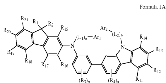
Formula 1A
